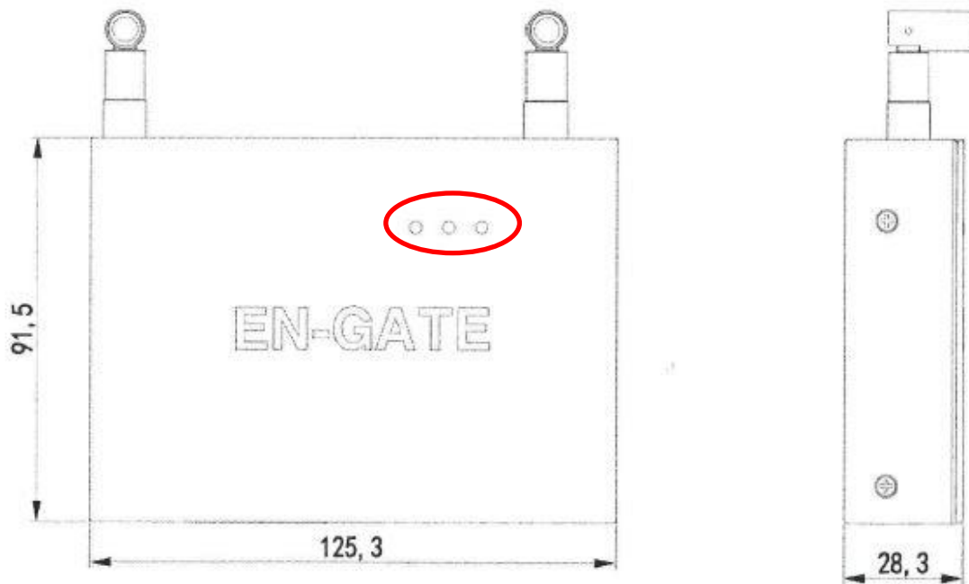
Figure 40 - Device dimensions
