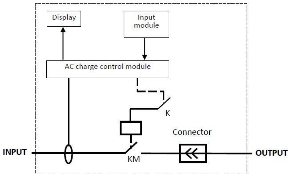
Figure 5 – Operating diagram of the charging station
