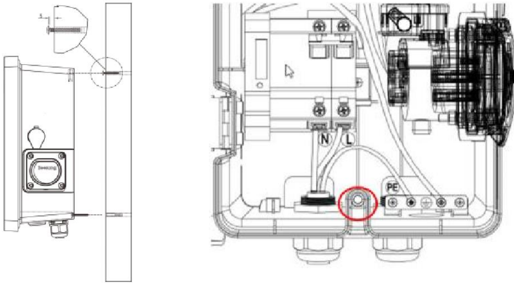
Figure 17 - Wall fixing
