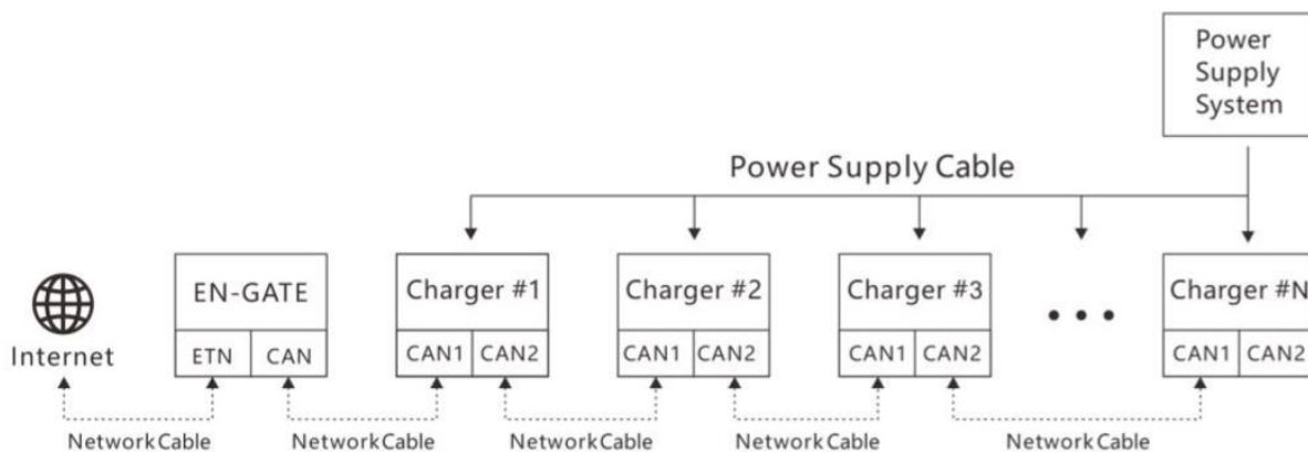
Figure 38 - Connection between ZSM-GATEWAY and the chargers
