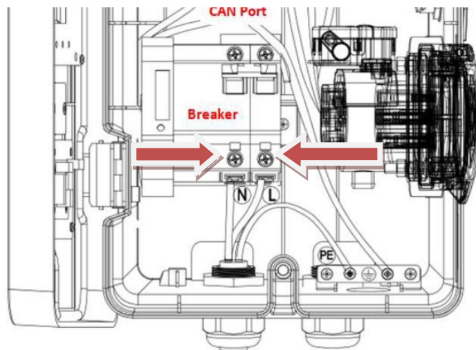
Figure 13 - Connecting the AC output cables (2)
