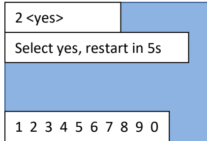
Figure 29 - Restart screen
