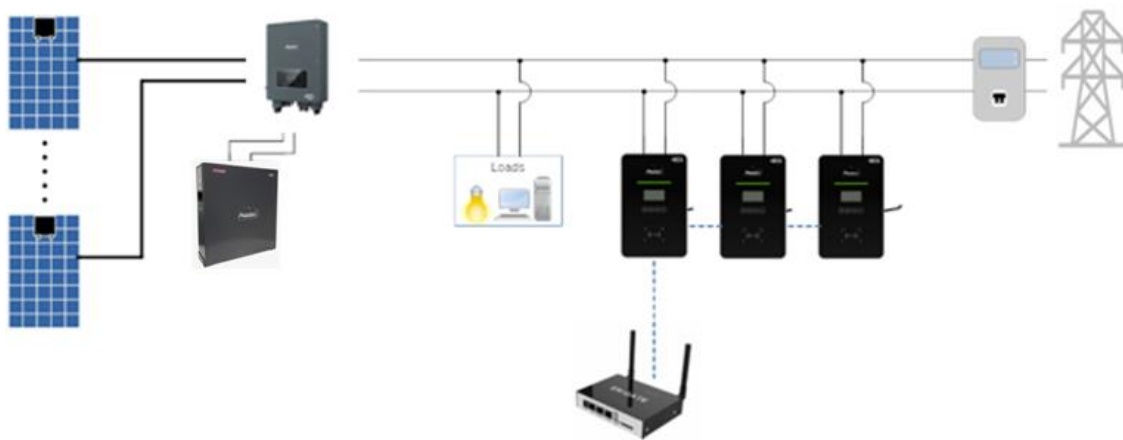
Figure 35 - Online mode
