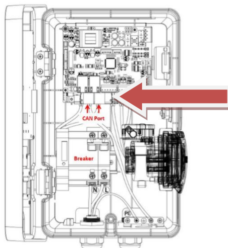
Figure 14 - Communication system
