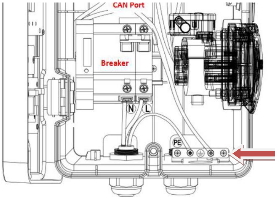
Figure 11 - Connecting the ground terminal
