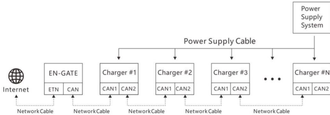
Figure 15 - Connecting the charging stations
