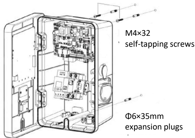
Figure 16 - Positioning of screws for wall mounting
