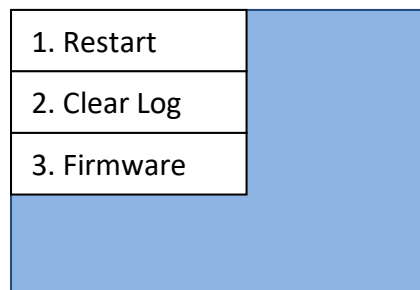
Figure 28 - Maintenance screen
