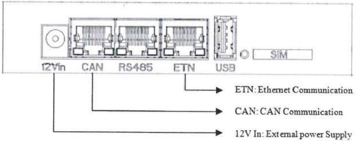
Figure 39 - Definition of inputs
