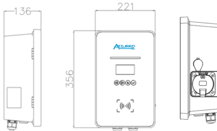
Figure 4 – Front and side view of the charging station
